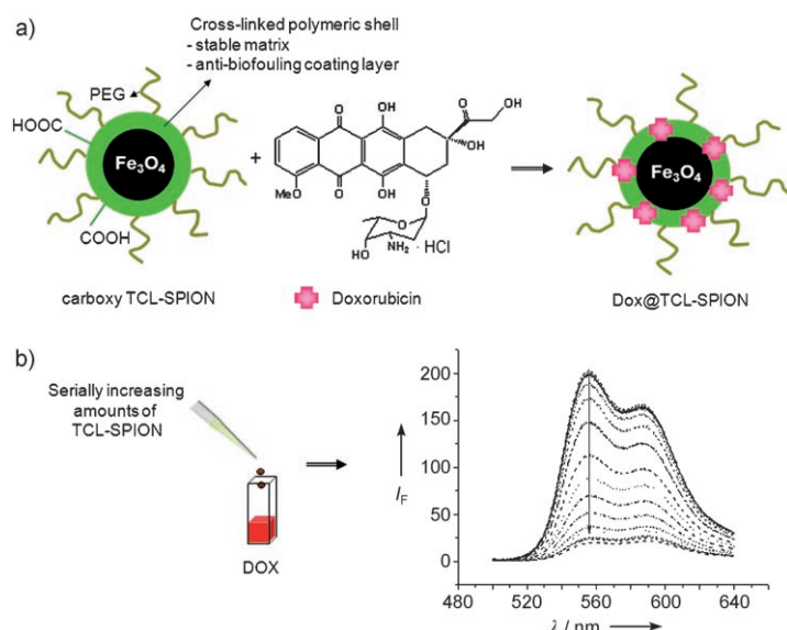
Figure 1. a) Formation of Dox@TCL-SPIONs. b) Fluorescence spectra of Dox solution ( 4\text{ }\mu\text{g} in 150\text{ }\mu\text{L} of 5% glucose solution) with increasing amounts of TCL-SPION (from top to bottom: 0.18, 0.37, 0.75, 1.5, 3, 6.25, 12.5, 25, 50, 70, 100, 130, 150, 180, 200, 220, and 250\text{ }\mu\text{g} ).
